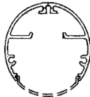
D116-2.0 - HR Hand rail extrusion
