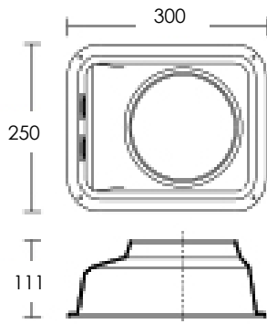
Housing for Concrete
